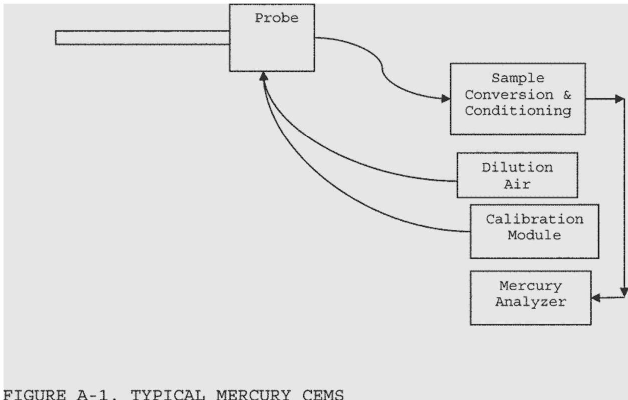
FIGURE A-1. TYPICAL MERCURY CEMS
